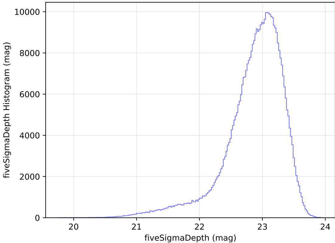
too_elab_r8_d2_giz_v3.4_10yrs WFD z band: fiveSigmaDepth Histogram
