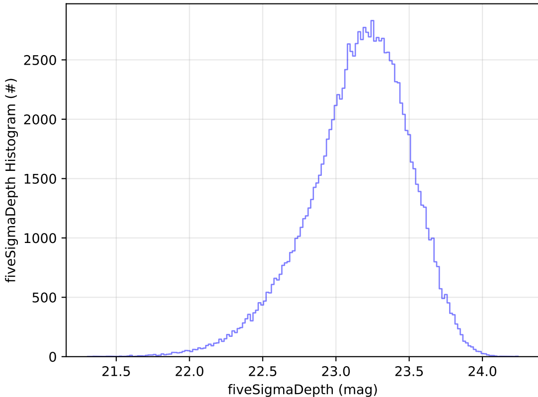
too_elab_r8_d2_giz_v3.4_10yrs WFD u band: fiveSigmaDepth Histogram
