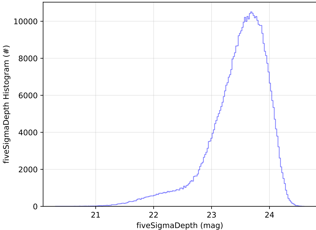
too_elab_r8_d2_giz_v3.4_10yrs WFD i band: fiveSigmaDepth Histogram
