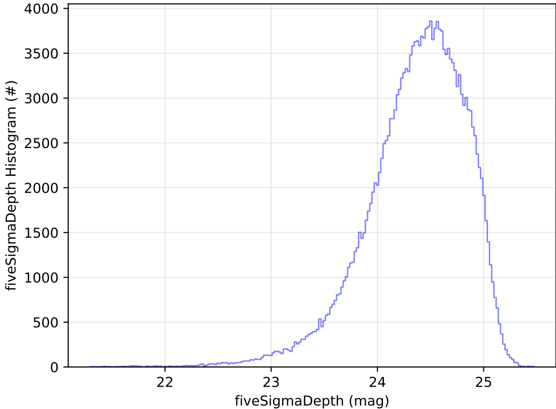
too_elab_r8_d2_giz_v3.4_10yrs WFD g band: fiveSigmaDepth Histogram
