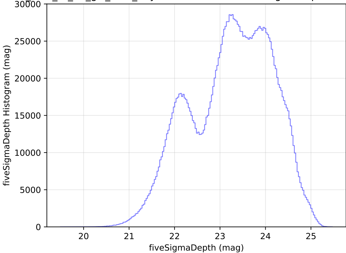
too_elab_r8_d2_giz_v3.4_10yrs WFD all bands: fiveSigmaDepth Histogram
