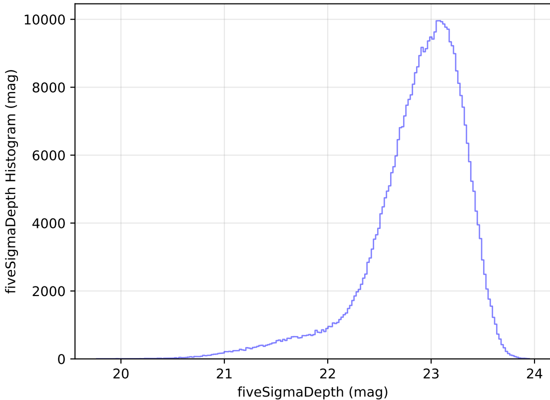
too_elab_r8_d2_giz_v3.4_10yrs All sky z band: fiveSigmaDepth Histogram
