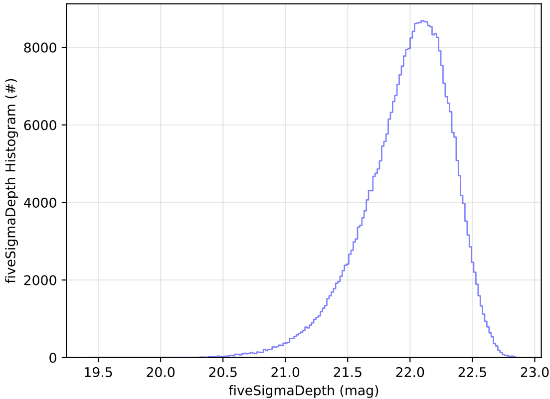
too_elab_r8_d2_giz_v3.4_10yrs All sky y band: fiveSigmaDepth Histogram
