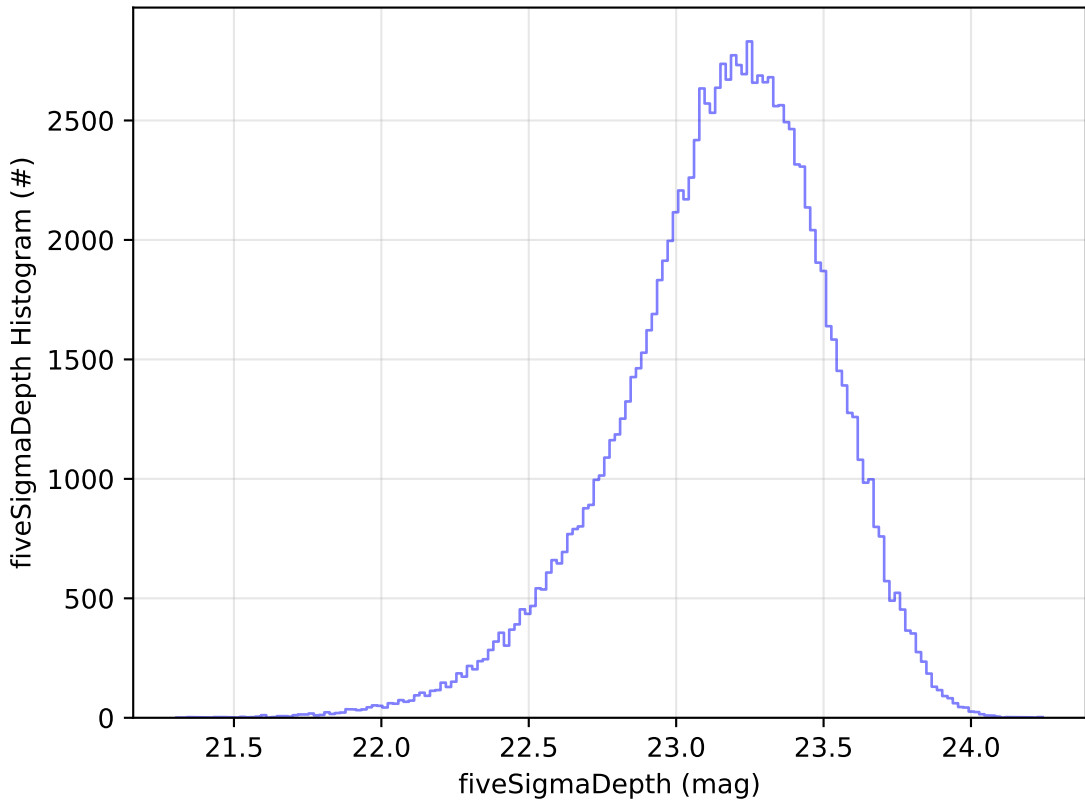
too_elab_r8_d2_giz_v3.4_10yrs All sky u band: fiveSigmaDepth Histogram
