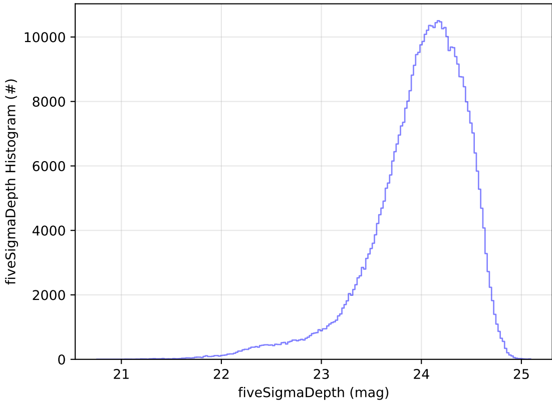
too_elab_r8_d2_giz_v3.4_10yrs All sky r band: fiveSigmaDepth Histogram
