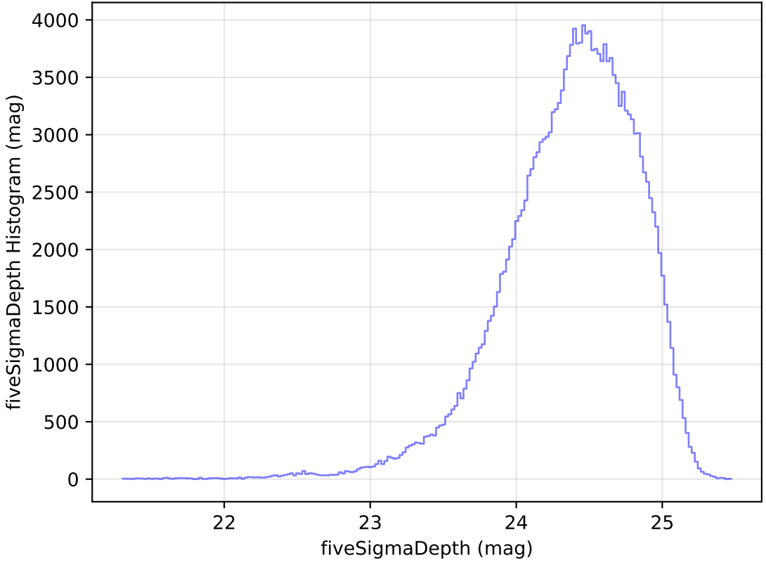
too_elab_r8_d2_giz_v3.4_10yrs All sky g band: fiveSigmaDepth Histogram
