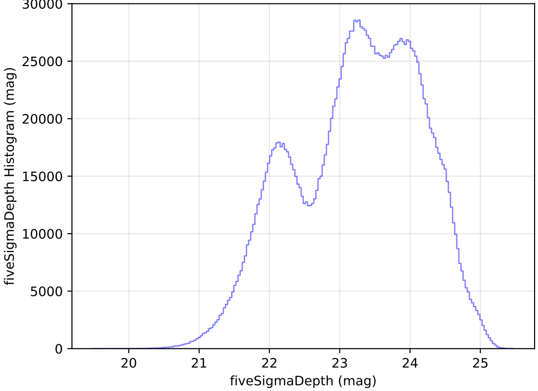
too_elab_r8_d2_giz_v3.4_10yrs All sky all bands: fiveSigmaDepth Histogram
