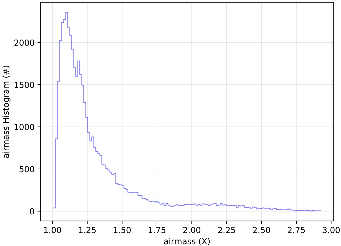
too_elab_r8_d2_giz_v3.4_10yrs Yr 1 z band: airmass Histogram
