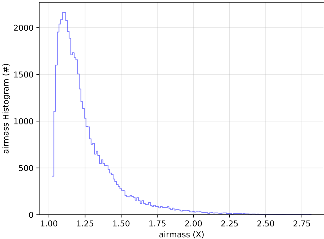
too_elab_r8_d2_giz_v3.4_10yrs Yr 1 y band: airmass Histogram
