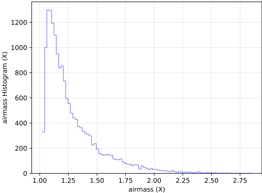
too_elab_r8_d2_giz_v3.4_10yrs Yr 1 u band: airmass Histogram
