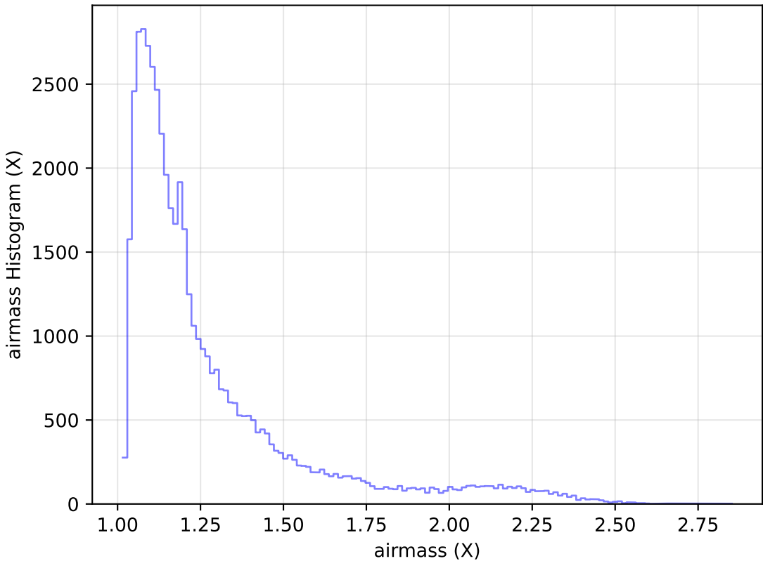
too_elab_r8_d2_giz_v3.4_10yrs Yr 1 r band: airmass Histogram
