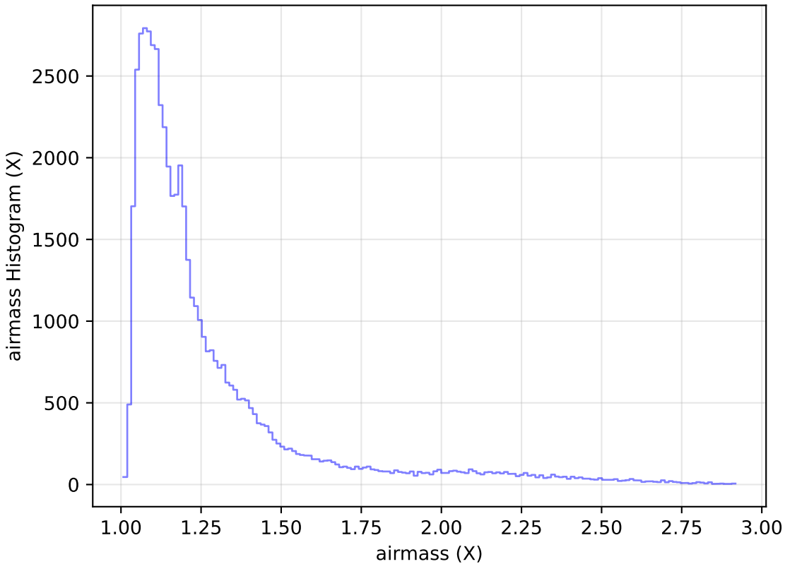
too_elab_r8_d2_giz_v3.4_10yrs Yr 1 i band: airmass Histogram
