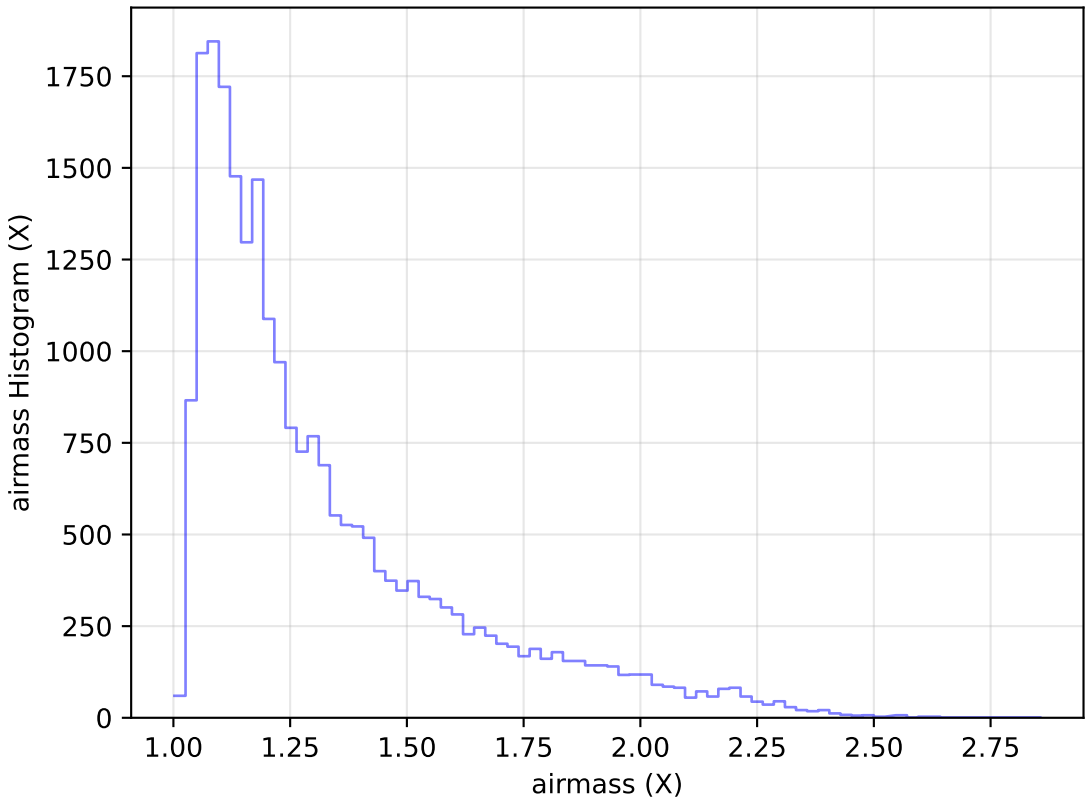
too_elab_r8_d2_giz_v3.4_10yrs Yr 1 g band: airmass Histogram
