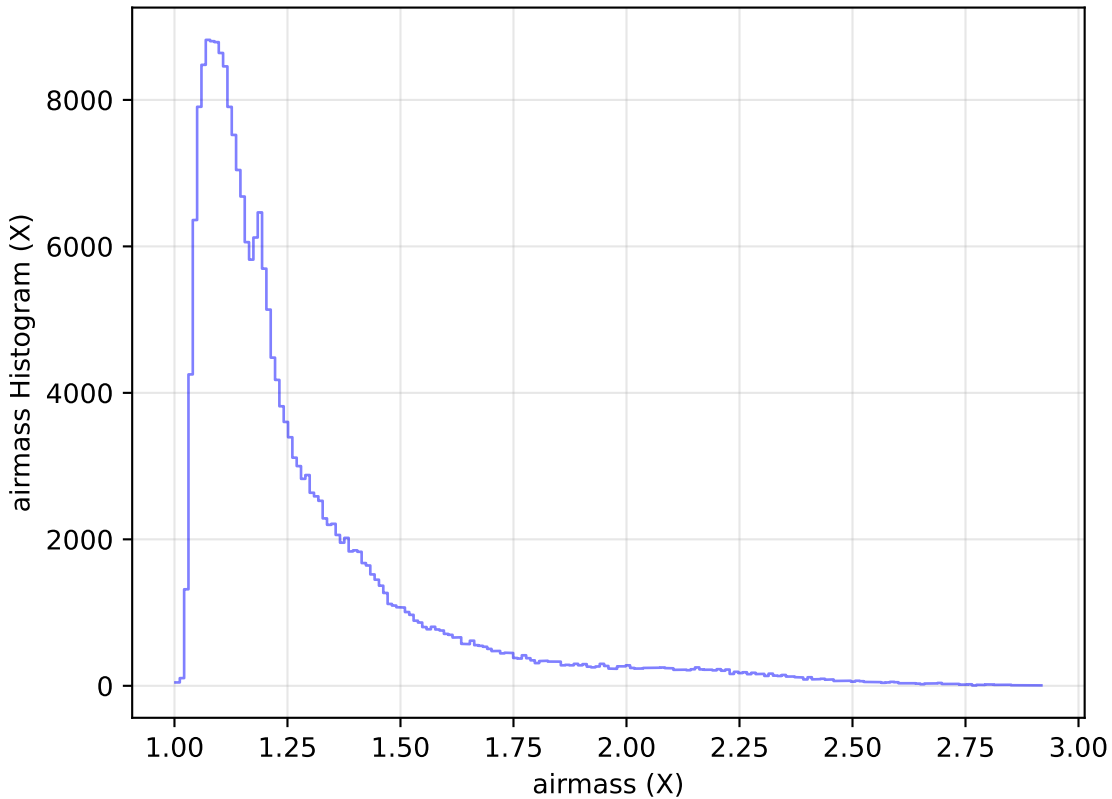
too_elab_r8_d2_giz_v3.4_10yrs Yr 1 all bands: airmass Histogram
