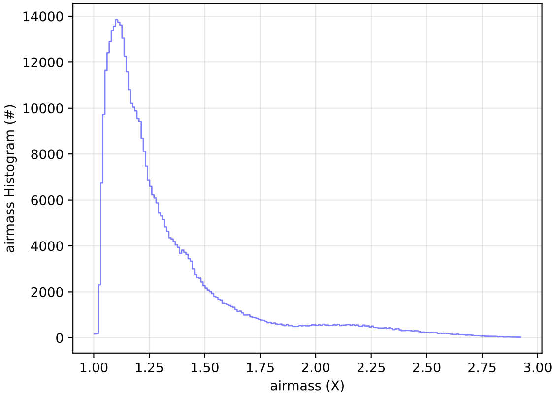
too_elab_r8_d2_giz_v3.4_10yrs WFD z band: airmass Histogram
