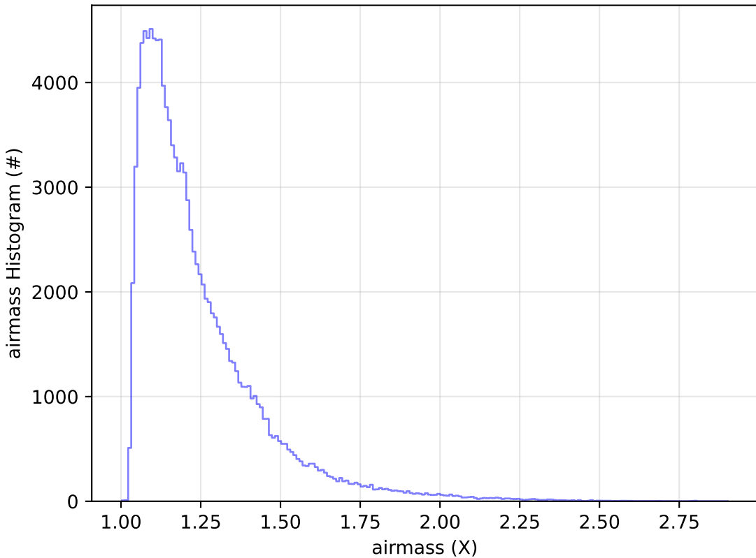
too_elab_r8_d2_giz_v3.4_10yrs WFD u band: airmass Histogram
