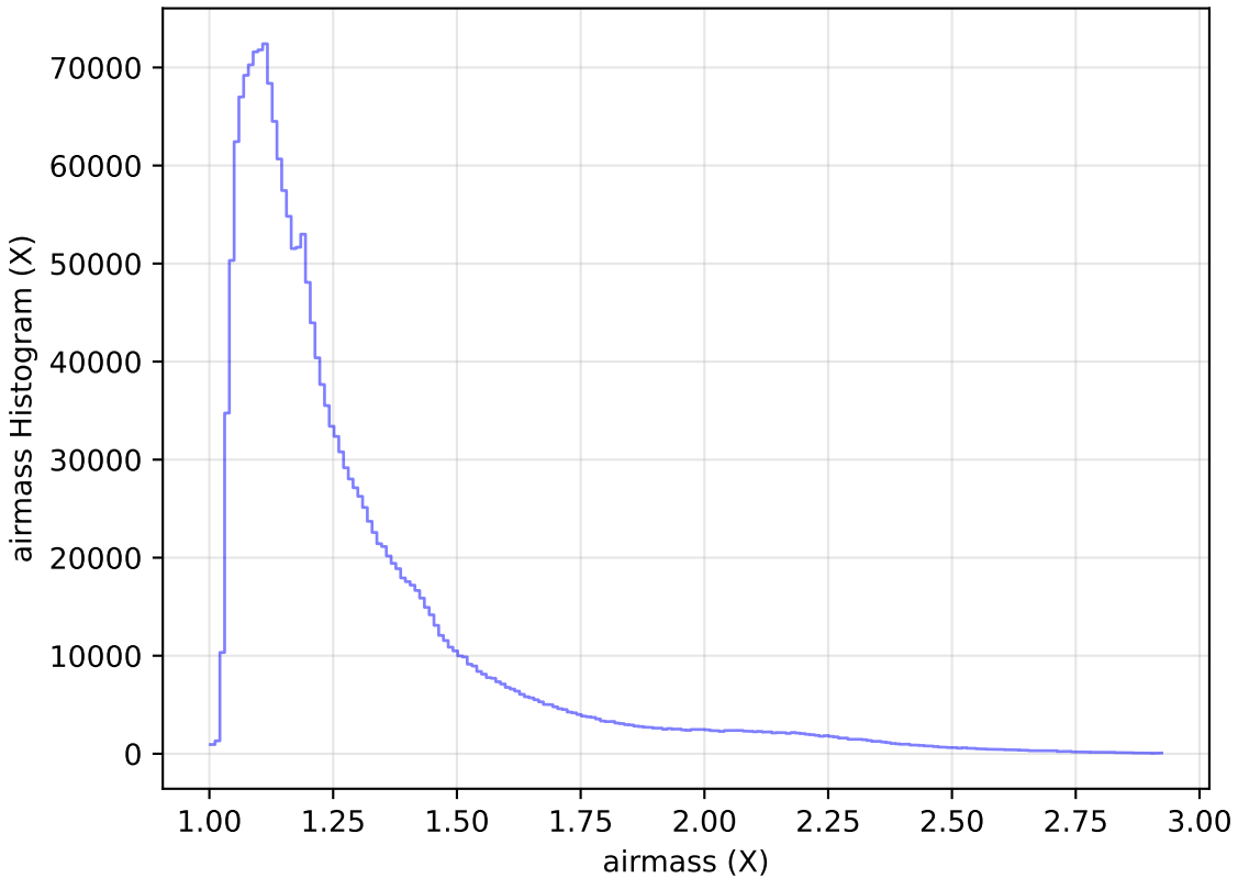
too_elab_r8_d2_giz_v3.4_10yrs WFD all bands: airmass Histogram
