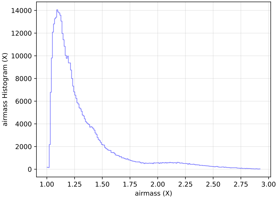
too_elab_r8_d2_giz_v3.4_10yrs All sky z band: airmass Histogram
