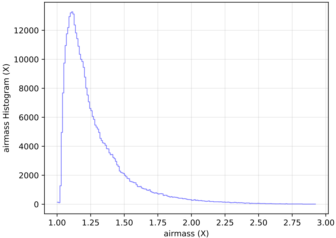
too_elab_r8_d2_giz_v3.4_10yrs All sky y band: airmass Histogram
