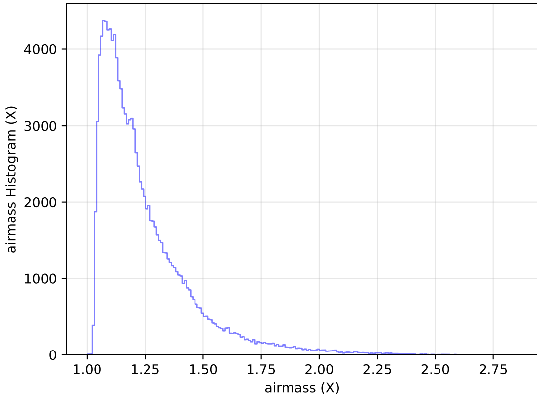
too_elab_r8_d2_giz_v3.4_10yrs All sky u band: airmass Histogram
