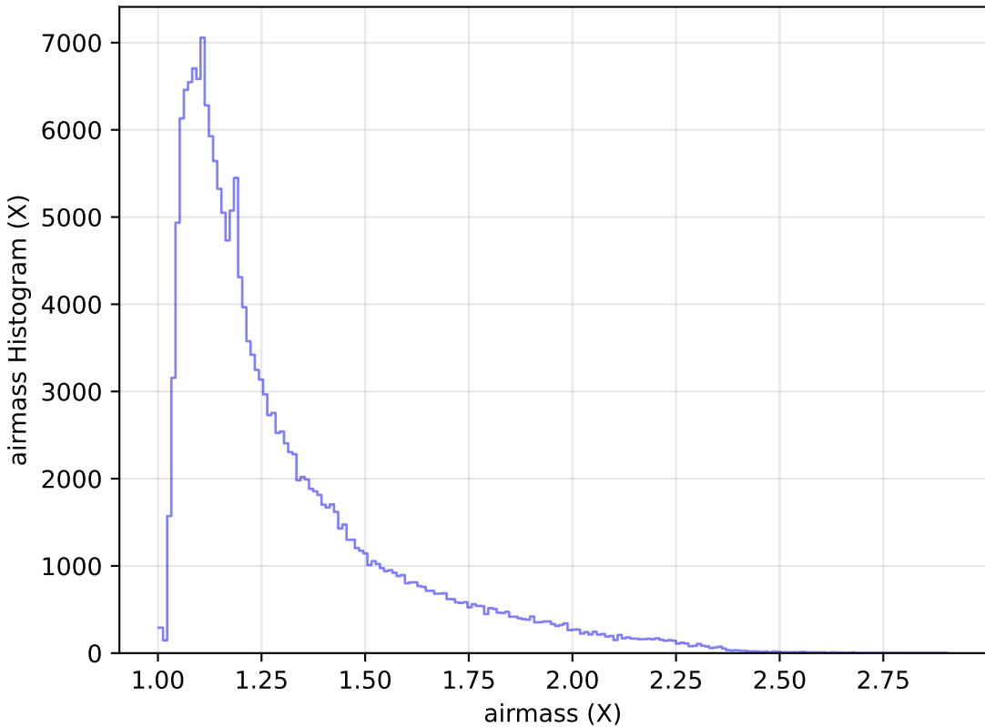
too_elab_r8_d2_giz_v3.4_10yrs All sky g band: airmass Histogram
