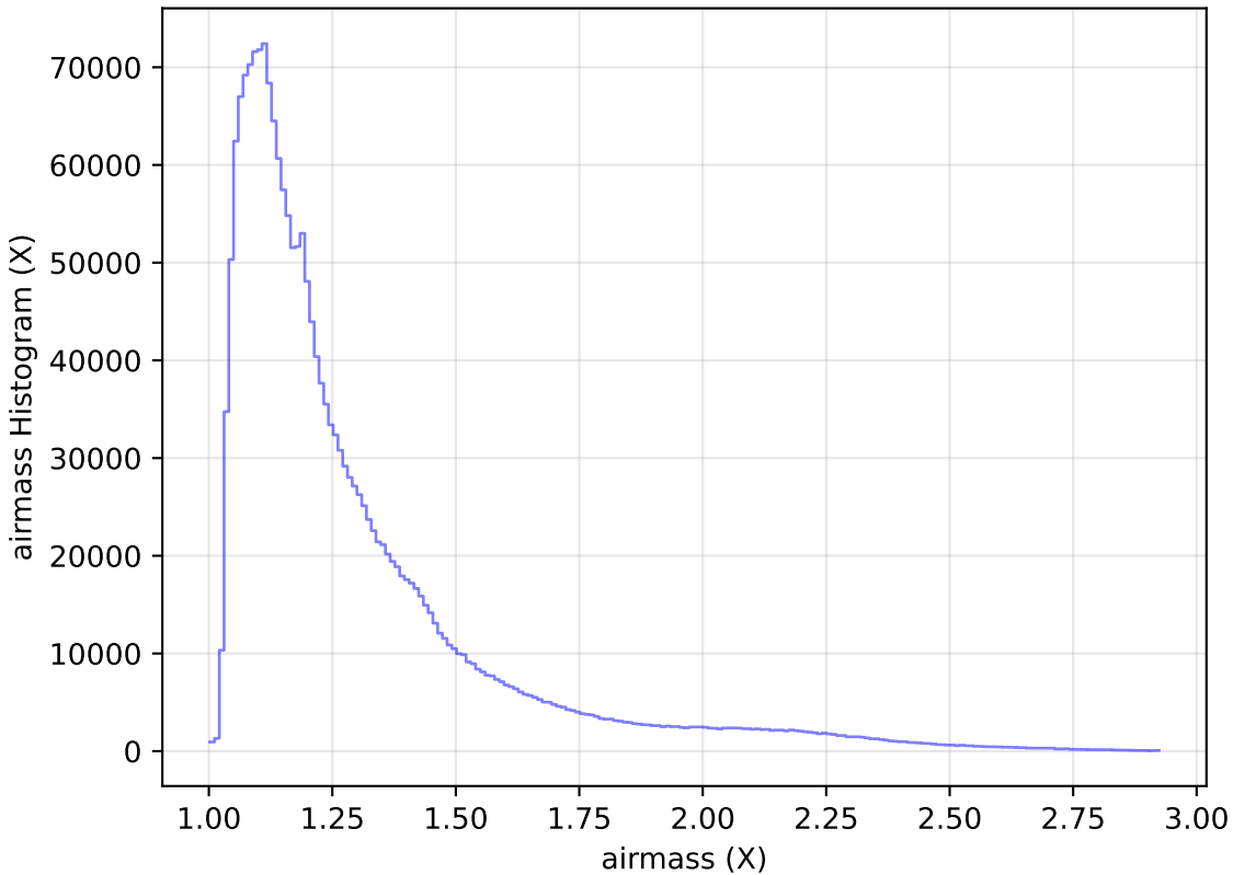
too_elab_r8_d2_giz_v3.4_10yrs All sky all bands: airmass Histogram
