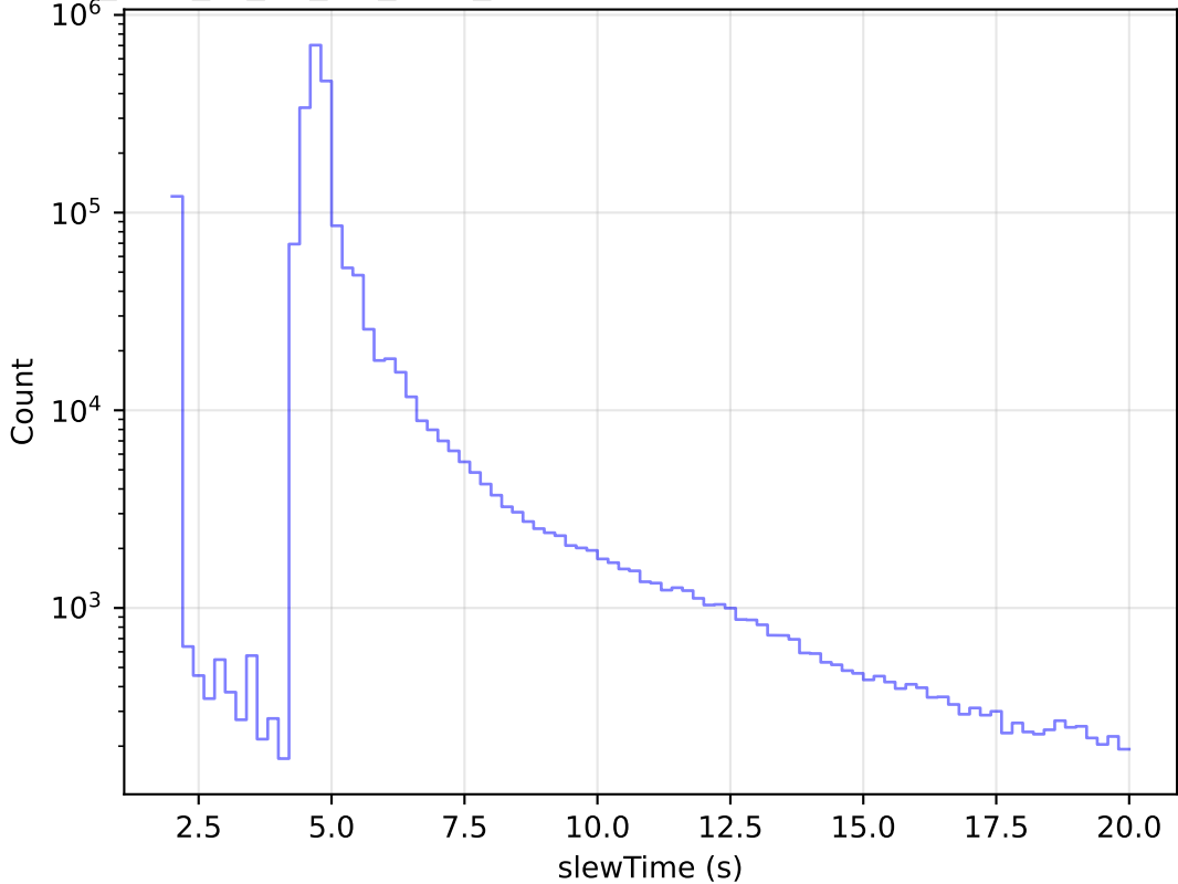
too_elab_r8_d2_giz_v3.4_10yrs All visits: Zoom Slew Time Histogram
