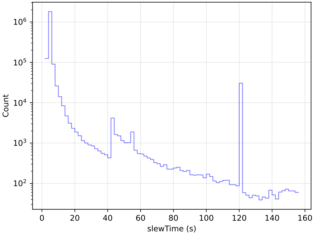
too_elab_r8_d2_giz_v3.4_10yrs All visits: Slew Time Histogram
