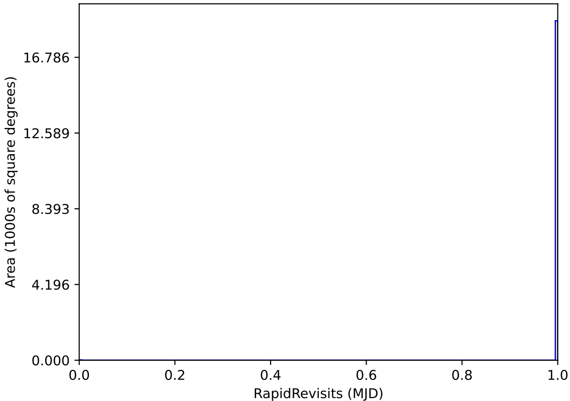
too_elab_r8_d2_giz_v3.4_10yrs WFD: RapidRevisits
