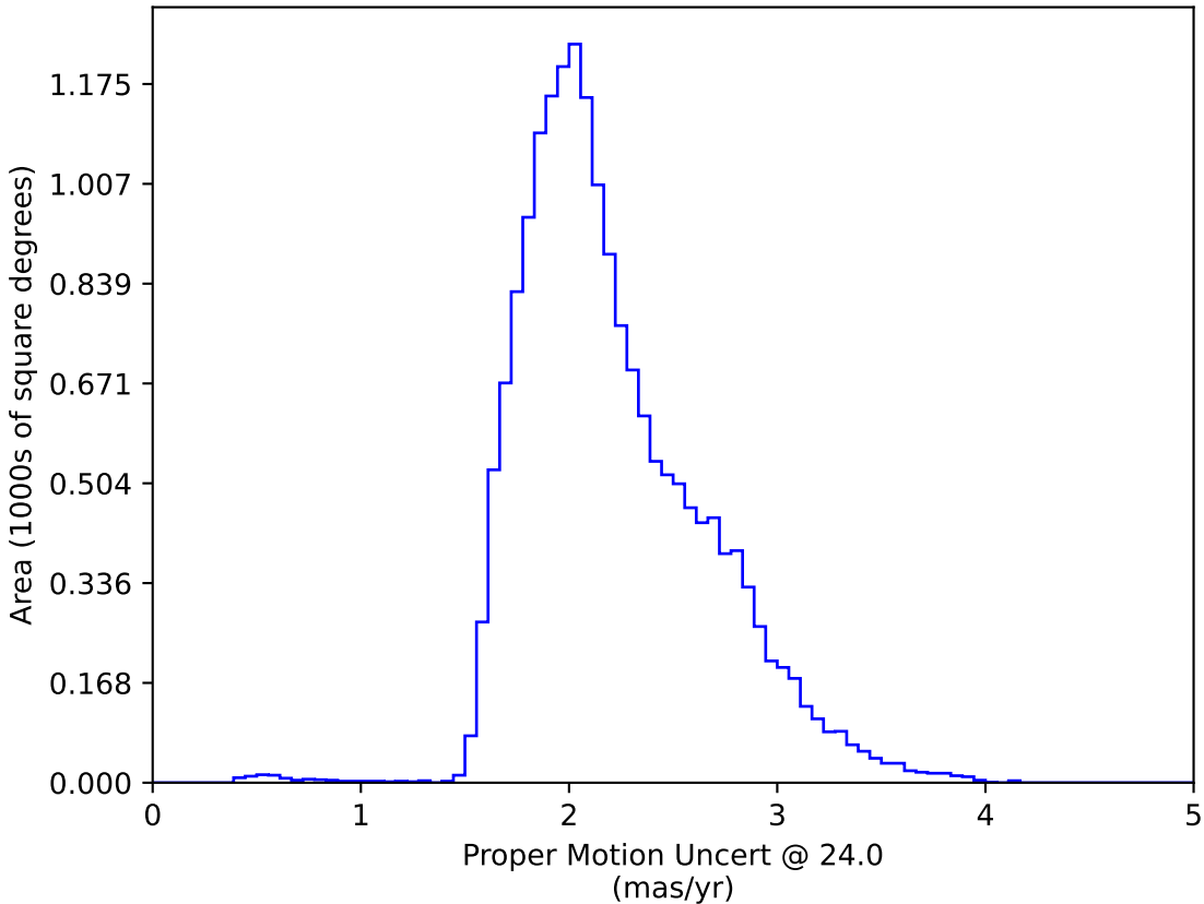
too_elab_r8_d2_giz_v3.4_10yrs WFD: Proper Motion Uncert @ 24.0
