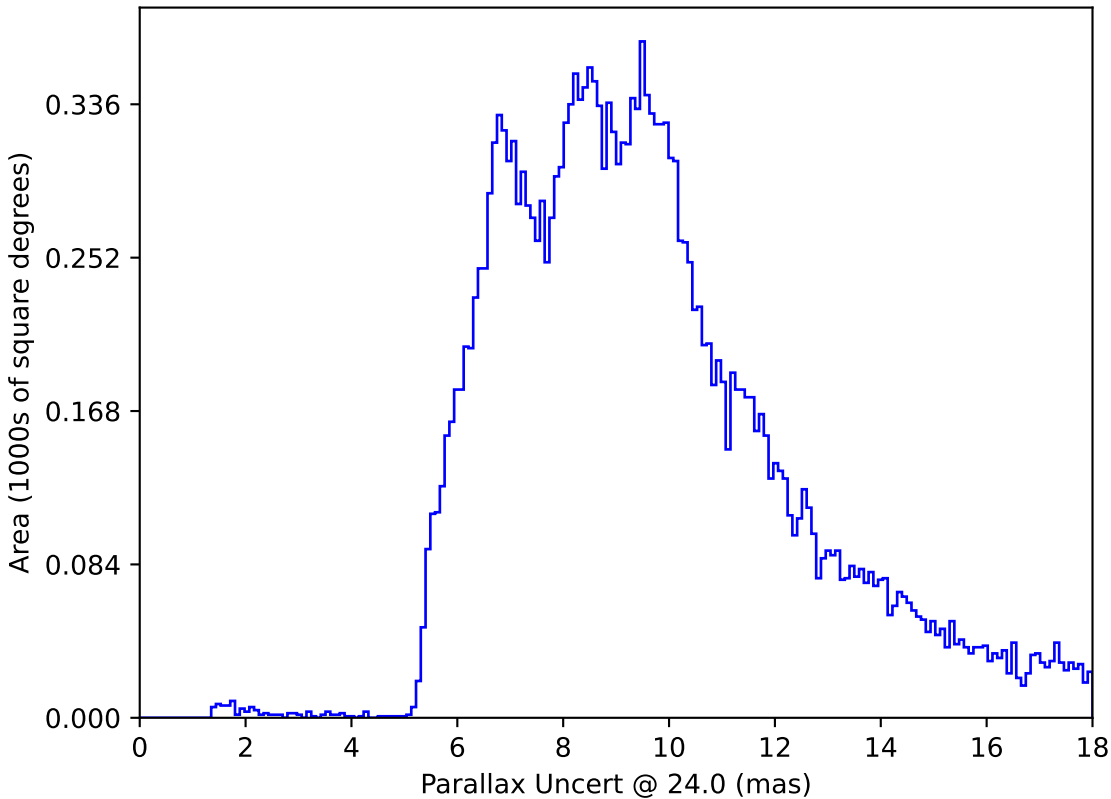
too_elab_r8_d2_giz_v3.4_10yrs All sky: Parallax Uncert @ 24.0
