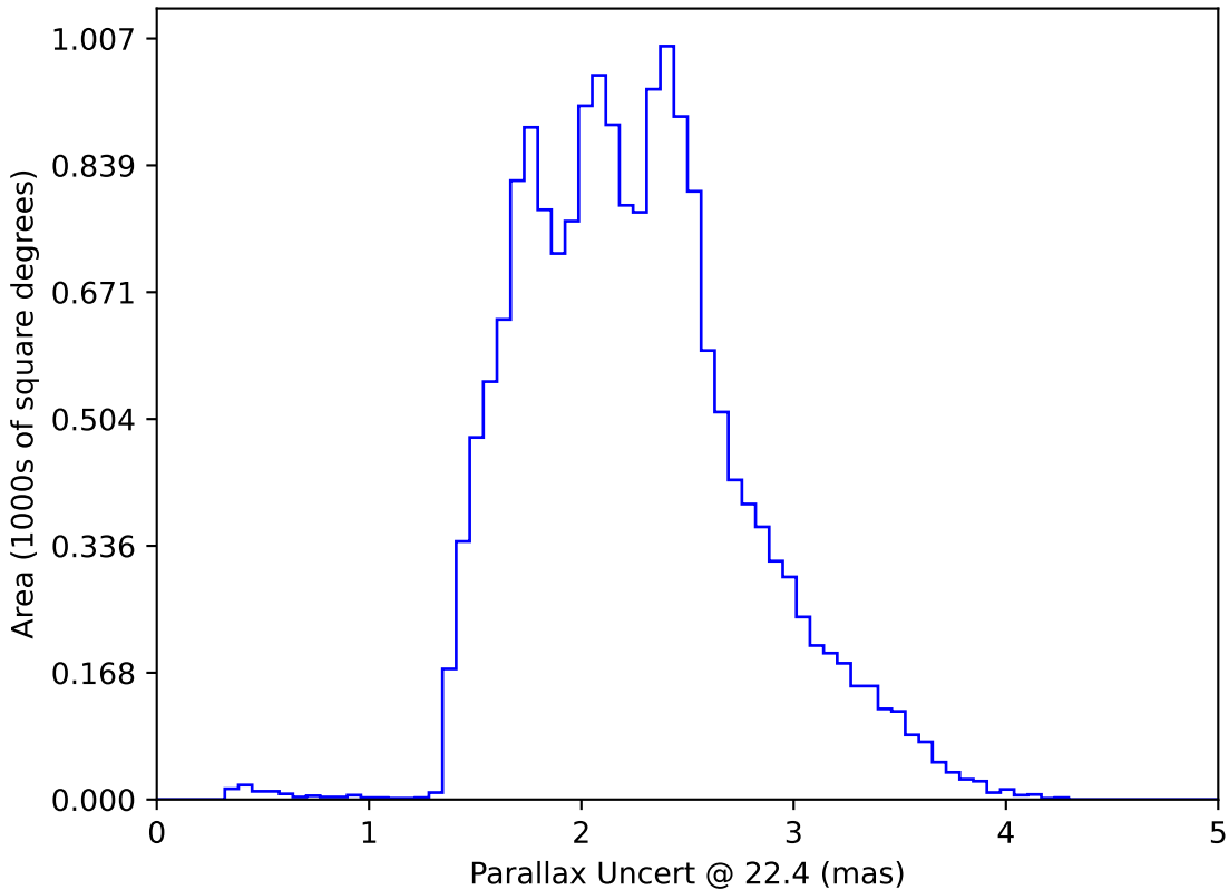
too_elab_r8_d2_giz_v3.4_10yrs WFD: Parallax Uncert @ 22.4
