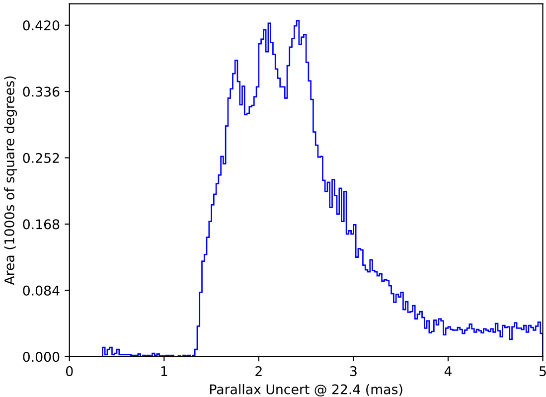
too_elab_r8_d2_giz_v3.4_10yrs All sky: Parallax Uncert @ 22.4
