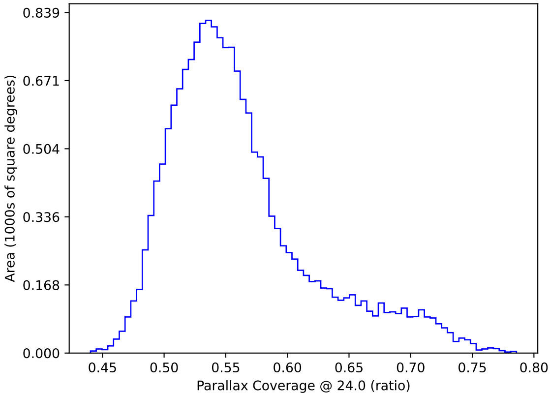
too_elab_r8_d2_giz_v3.4_10yrs WFD: Parallax Coverage @ 24.0
