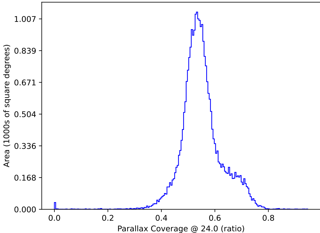
too_elab_r8_d2_giz_v3.4_10yrs All sky: Parallax Coverage @ 24.0
