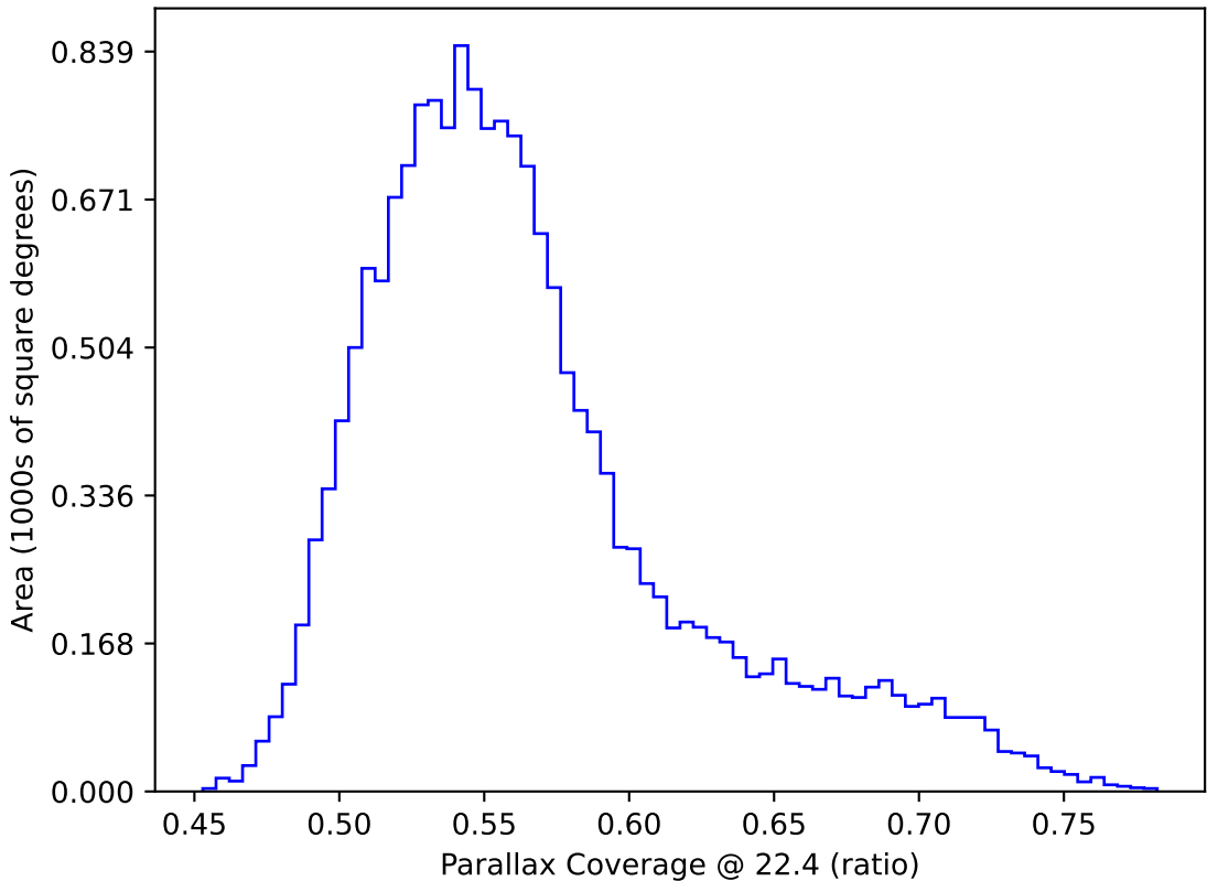
too_elab_r8_d2_giz_v3.4_10yrs WFD: Parallax Coverage @ 22.4
