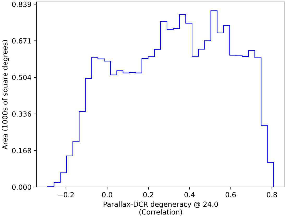
too_elab_r8_d2_giz_v3.4_10yrs WFD: Parallax-DCR degeneracy @ 24.0
