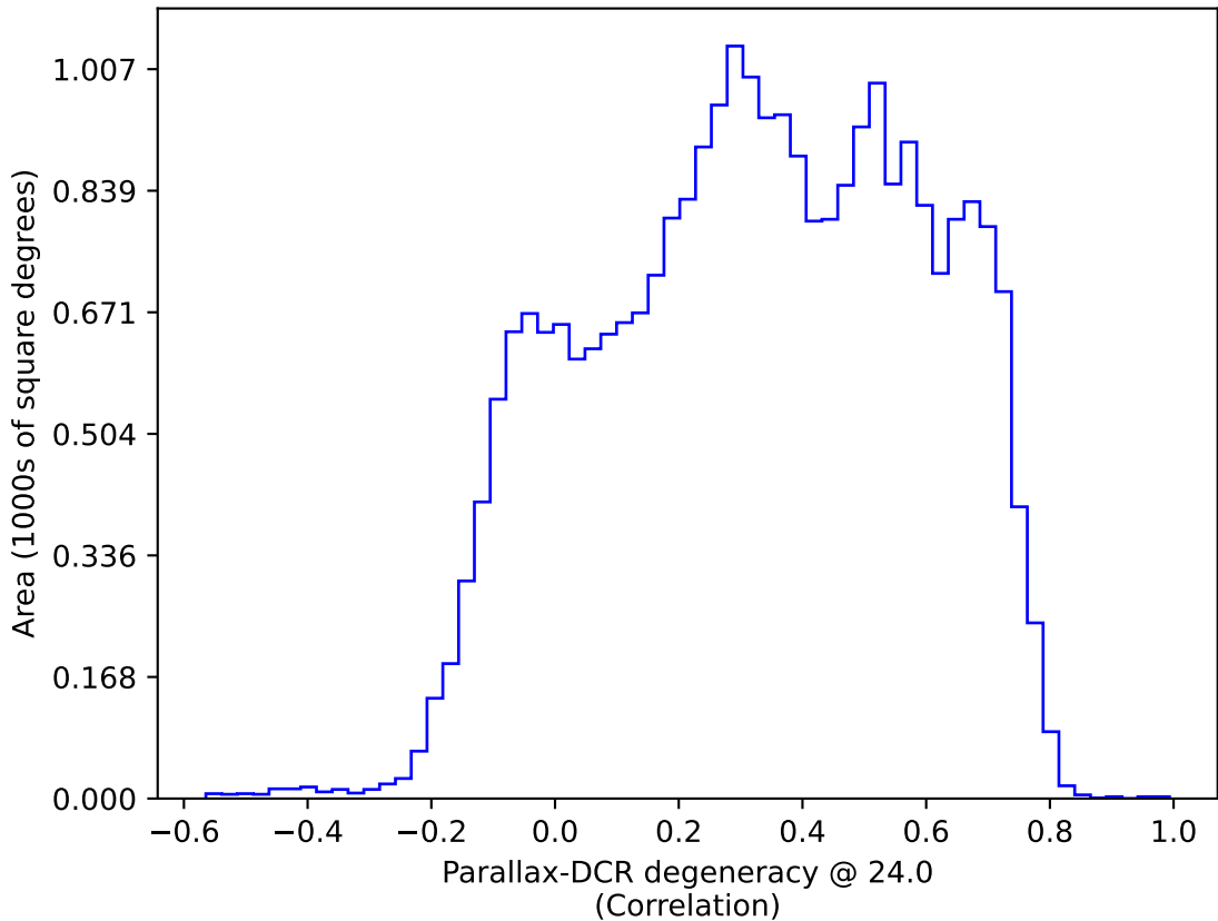
too_elab_r8_d2_giz_v3.4_10yrs All sky: Parallax-DCR degeneracy @ 24.0
