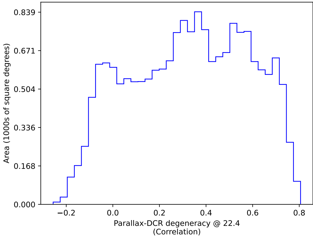
too_elab_r8_d2_giz_v3.4_10yrs WFD: Parallax-DCR degeneracy @ 22.4
