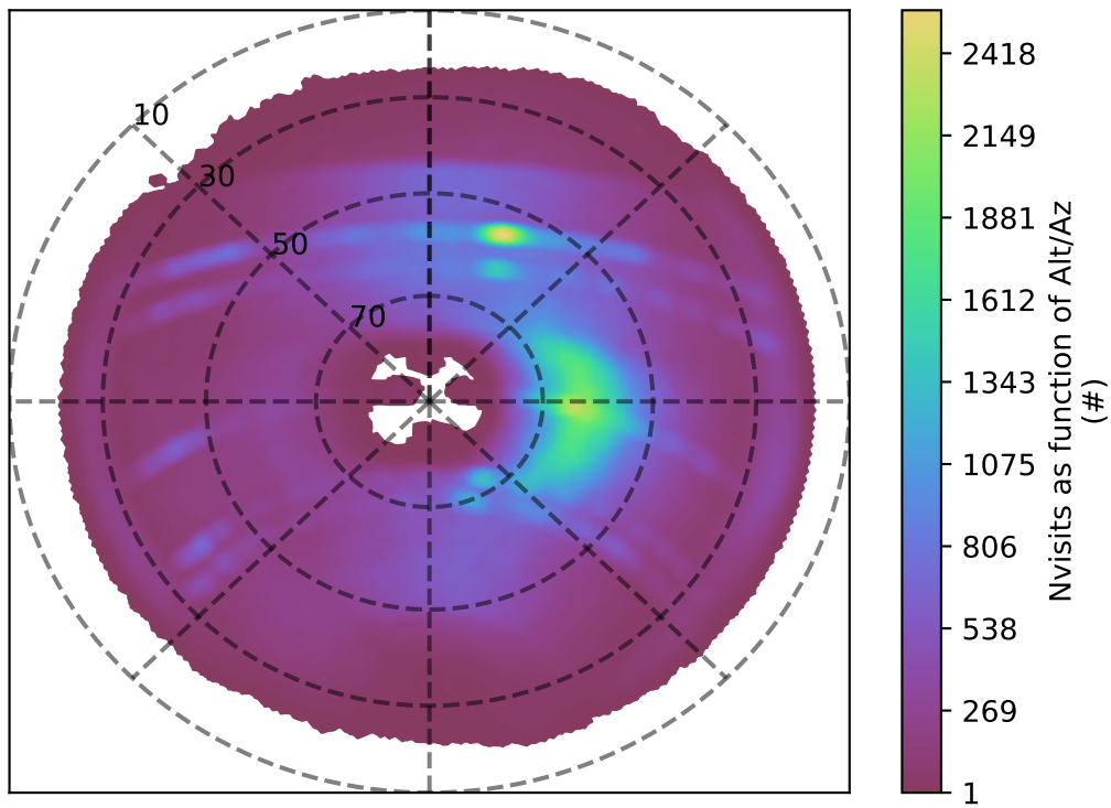
too_elab_r8_d2_giz_v3.4_10yrs z band: Nvisits as function of Alt/Az
