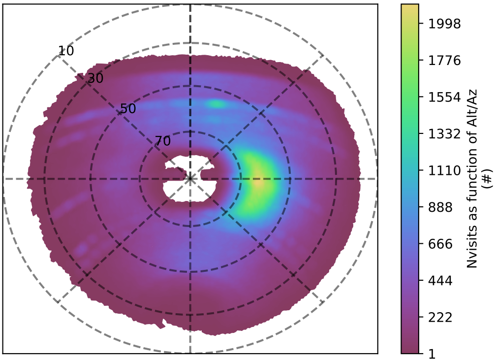
too_elab_r8_d2_giz_v3.4_10yrs y band: Nvisits as function of Alt/Az
