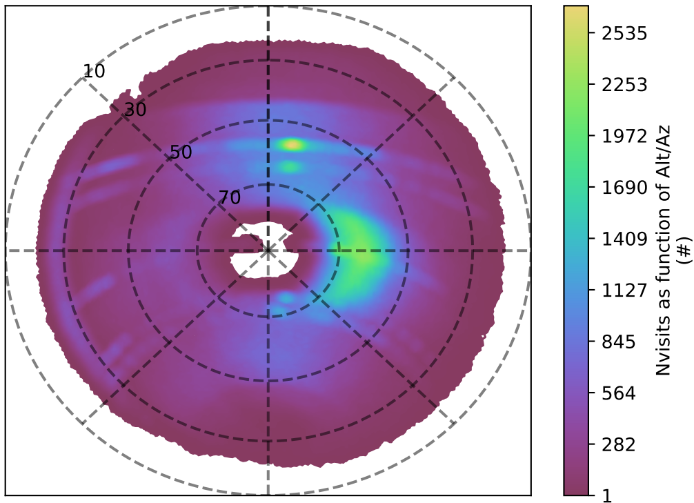
too_elab_r8_d2_giz_v3.4_10yrs r band: Nvisits as function of Alt/Az
