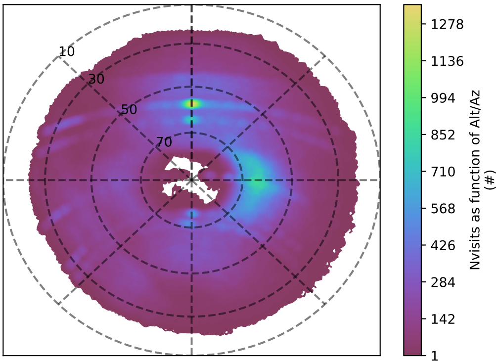
too_elab_r8_d2_giz_v3.4_10yrs g band: Nvisits as function of Alt/Az
