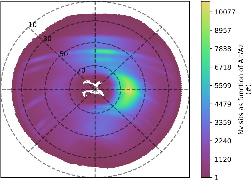
too_elab_r8_d2_giz_v3.4_10yrs all bands: Nvisits as function of Alt/Az
