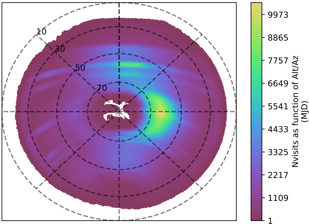
too_elab_r8_d2_giz_v3.4_10yrs all bands: Nvisits as function of Alt/Az
