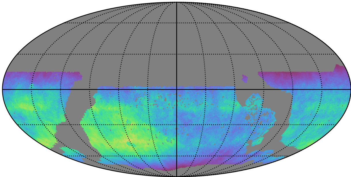
too_elab_r8_d2_giz_v3.4_10yrs WFD z band: Normalized Teff
