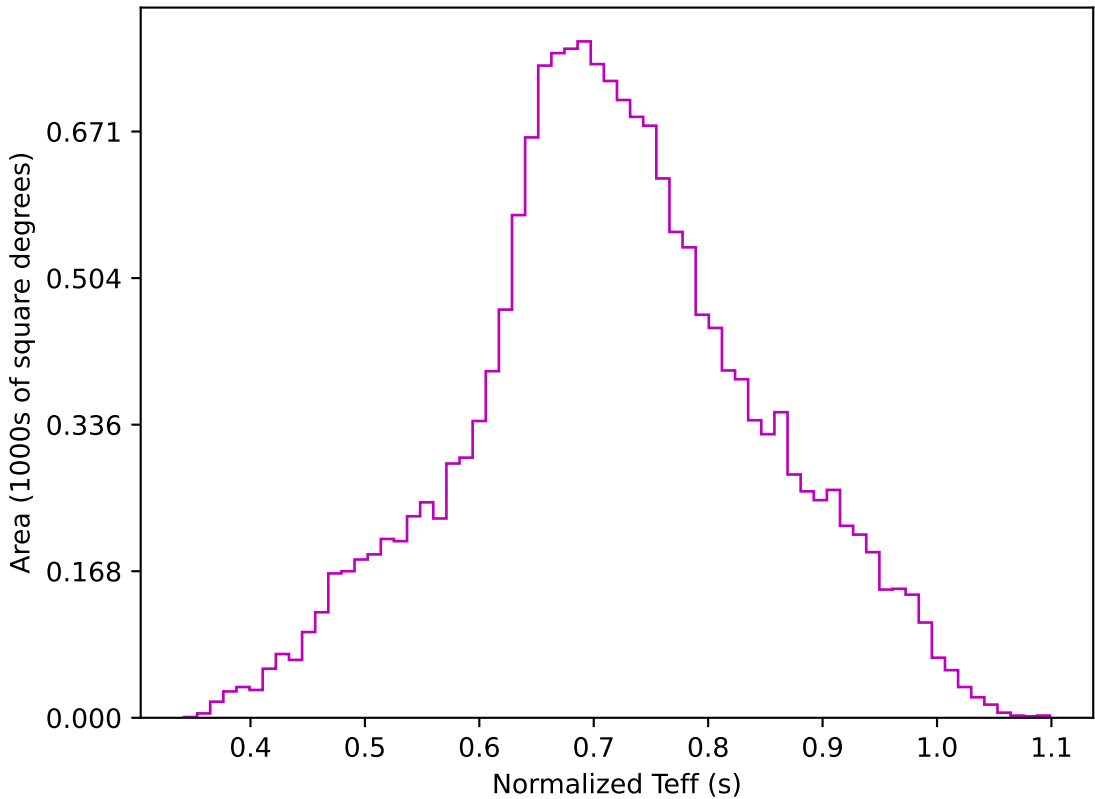
too_elab_r8_d2_giz_v3.4_10yrs WFD z band: Normalized Teff
