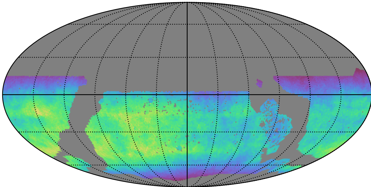
too_elab_r8_d2_giz_v3.4_10yrs WFD y band: Normalized Teff
