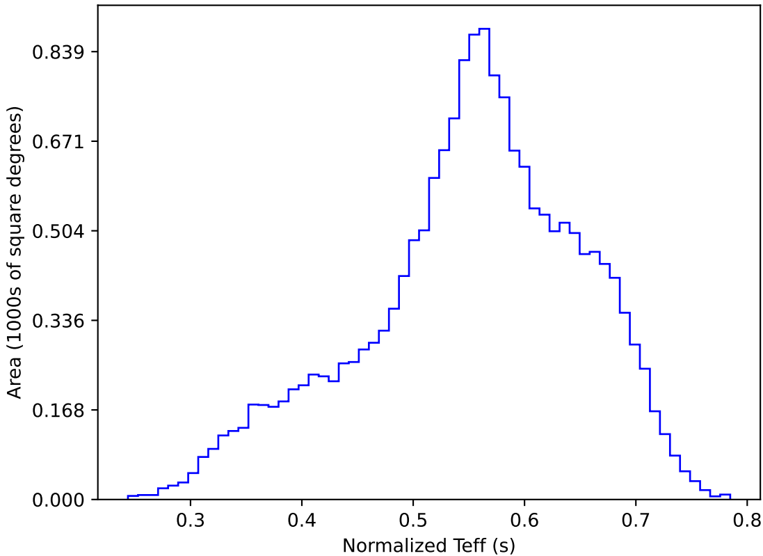
too_elab_r8_d2_giz_v3.4_10yrs WFD y band: Normalized Teff
