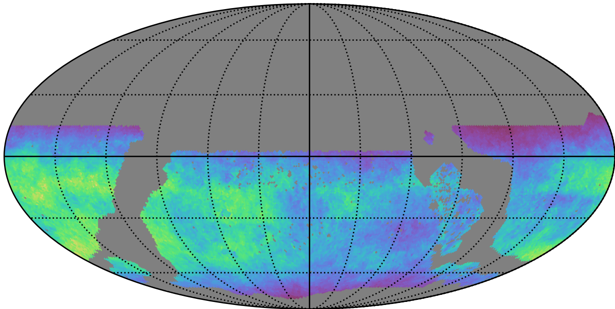
too_elab_r8_d2_giz_v3.4_10yrs WFD u band: Normalized Teff
