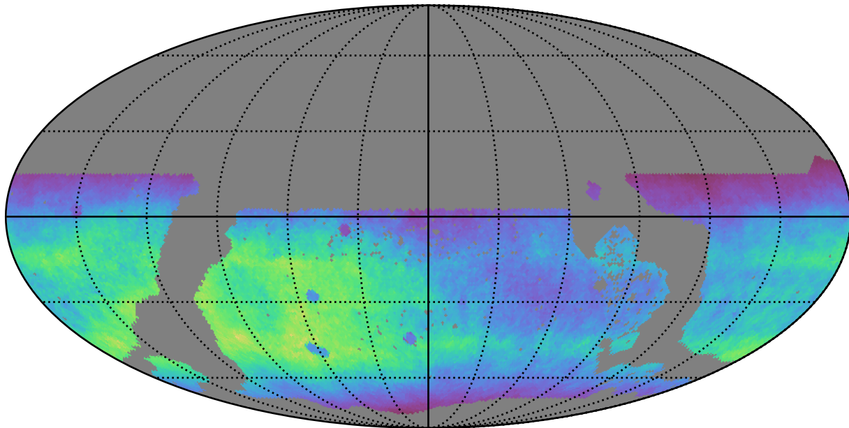
too_elab_r8_d2_giz_v3.4_10yrs WFD r band: Normalized Teff
